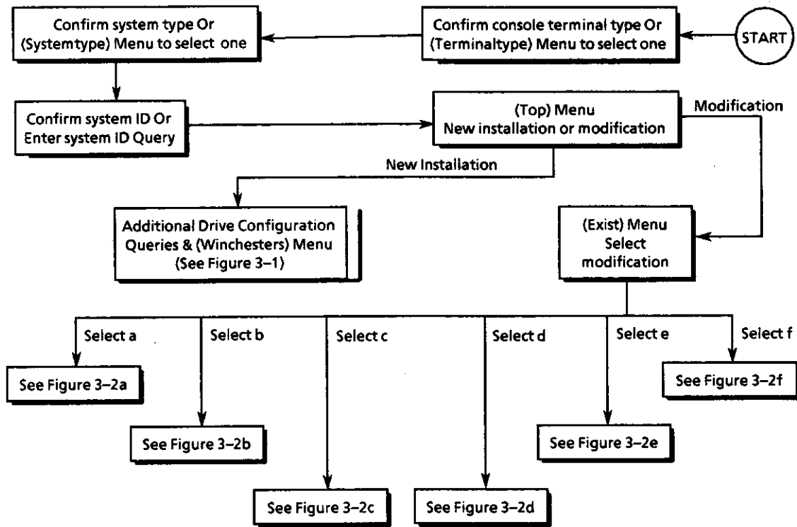
Figure 3-2. Reconfiguring An Existing System
