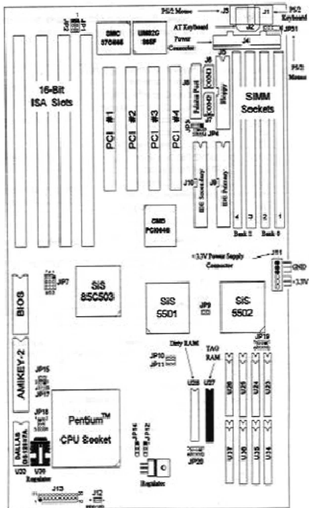
Figure 3-1. SIS4P AIO Mainboard Layout
