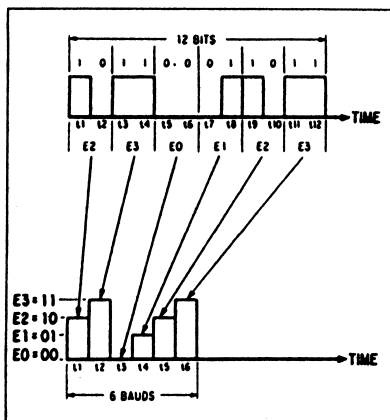
Figure 6. Bauds vs. Bits
