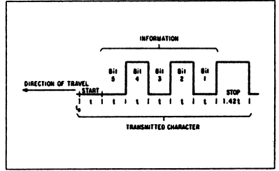
Figure 4. Asynchronous Signal
