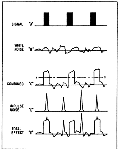
Figure 7. Effect of White Noise
