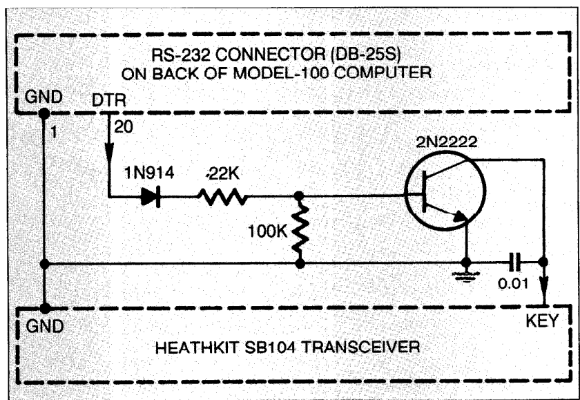
The article "Hello Rangoon" ( Portable 100 , November, 1985) describes an interface between a Model 100 and a Heathkit SB104 transceiver for sending CW. This is the schematic of that interface. The transmitter is turned on by +5 volts at pin 20 (DTR) of the computer's RS-232 port.
