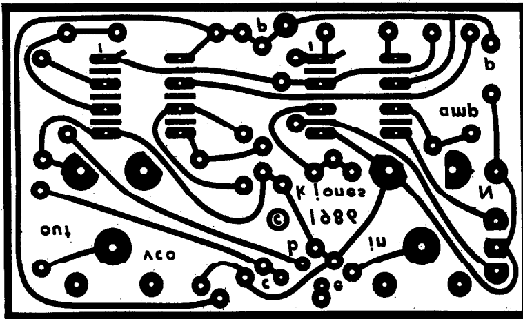
Circuit board layout seen from component side.
