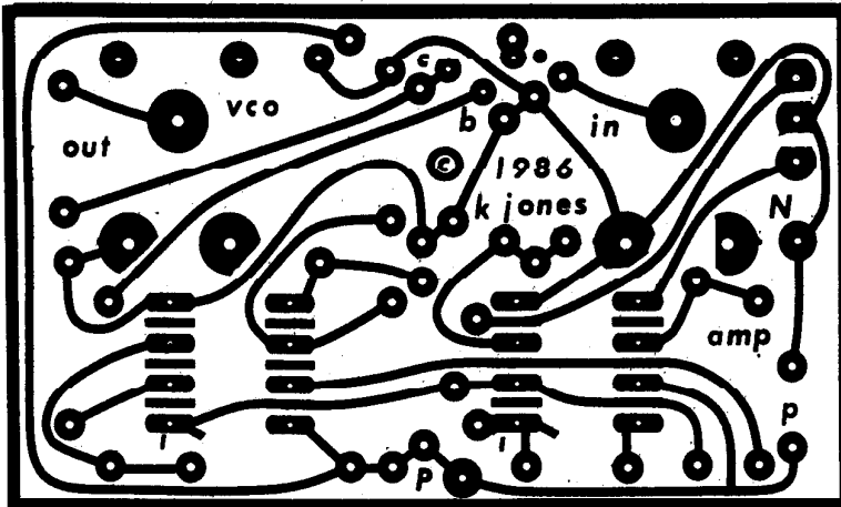
Circuit board layout seen front side.
