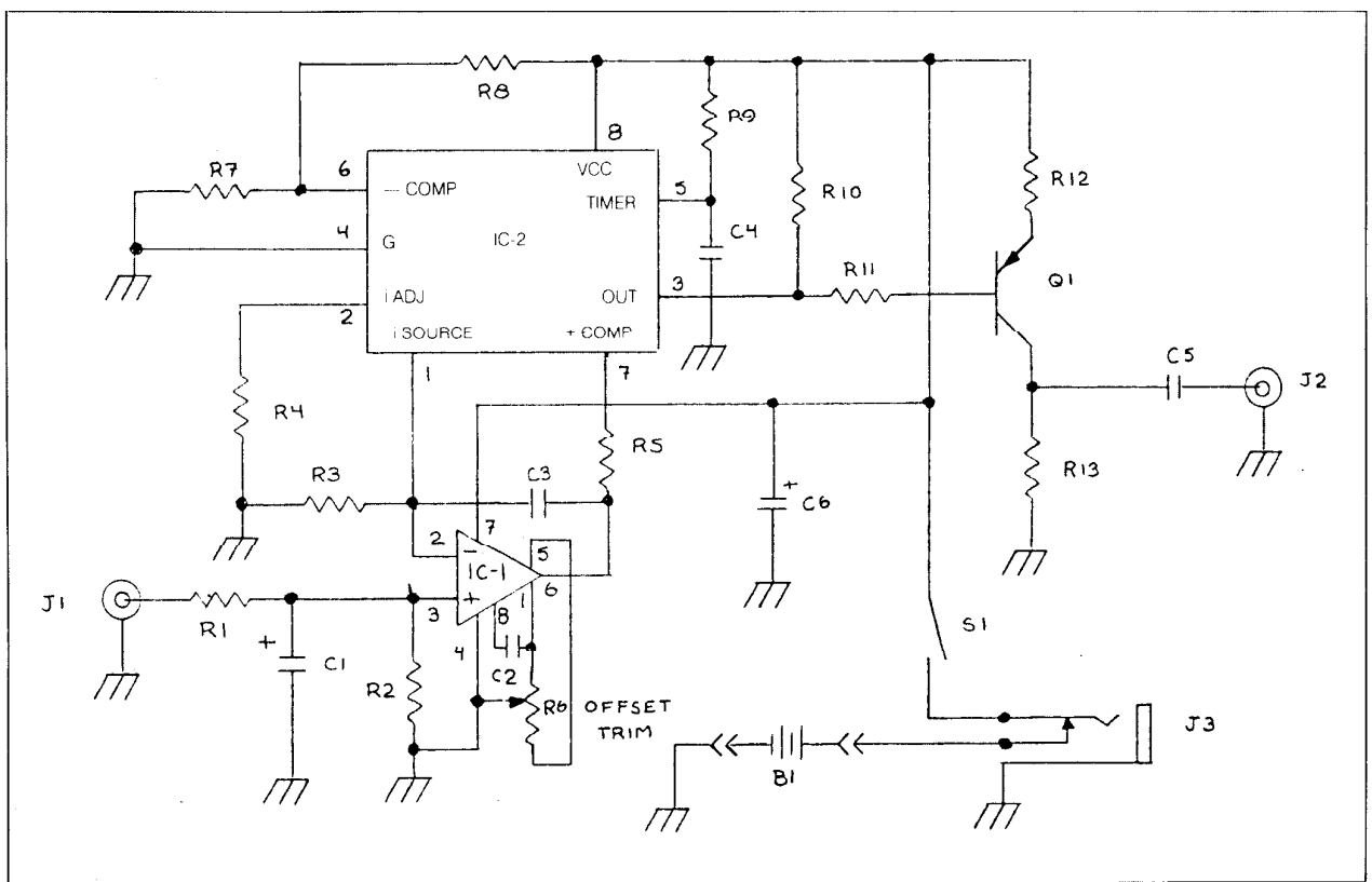
Schematic of the Datamite VCO unit.
