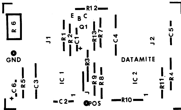
Component location overlay for top of board.
